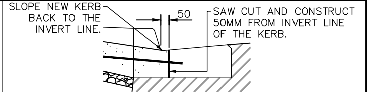
SAWCUT DETAIL
