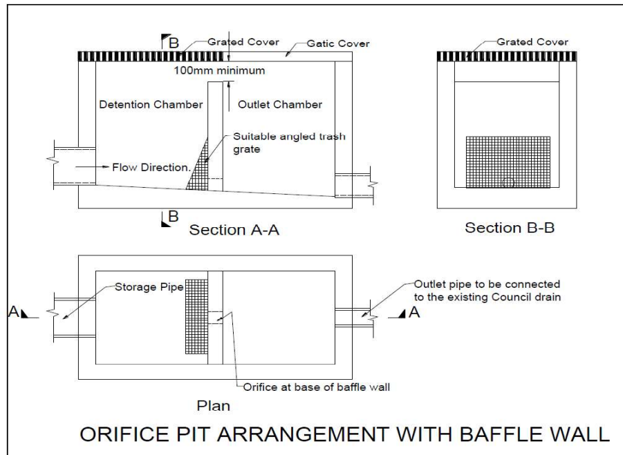
Figure 3 – Orifice Pit detail
