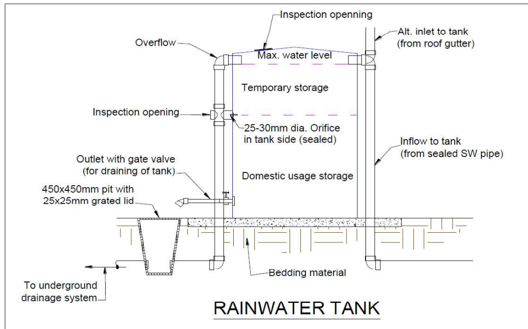
Figure 2 – Rainwater tank detail
