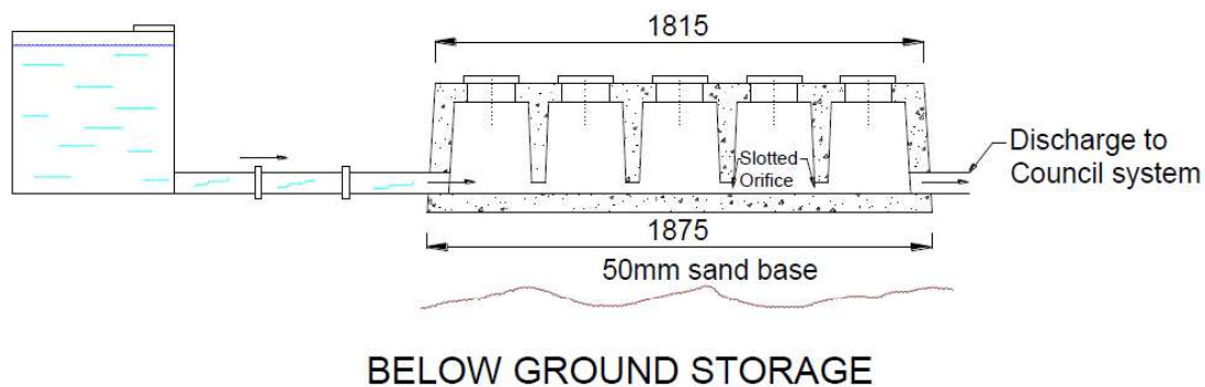
Figure 5 – Below ground multi-cell system
