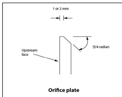
Figure 4 – Orifice plate detail
