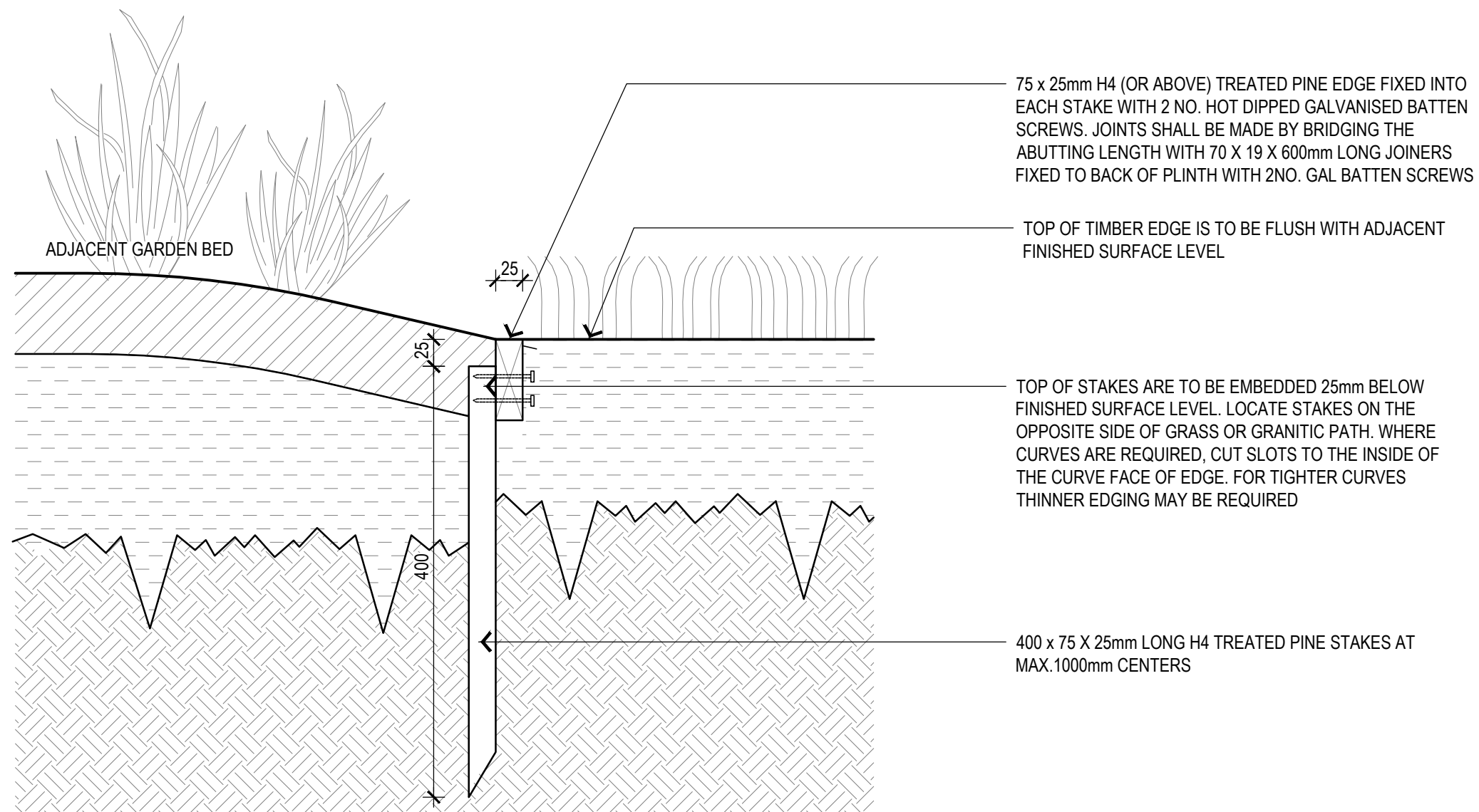
1 TIMBER EDGE - CROSS SECTION 1:5
