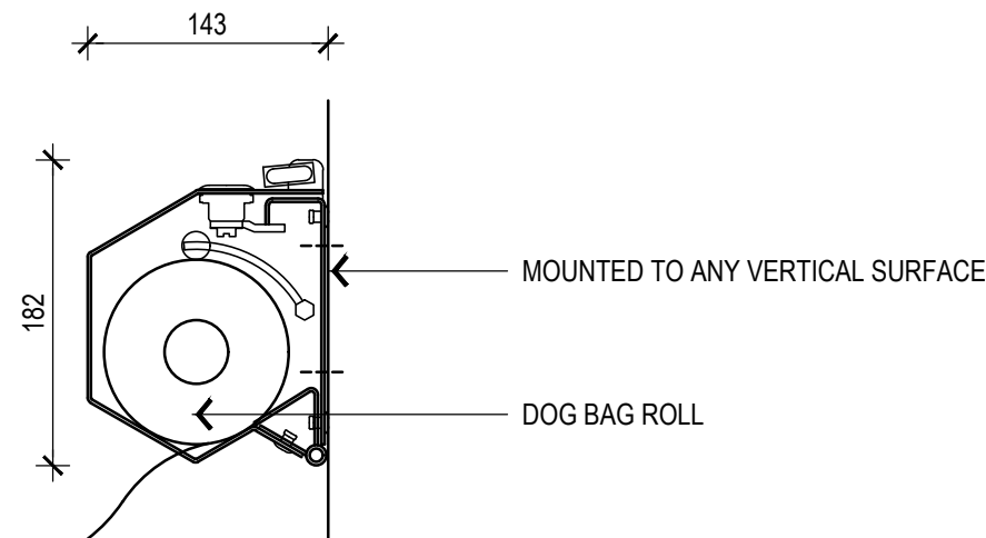
3 - DOG BAG DISPENSER CROSS SECTION 1:5
